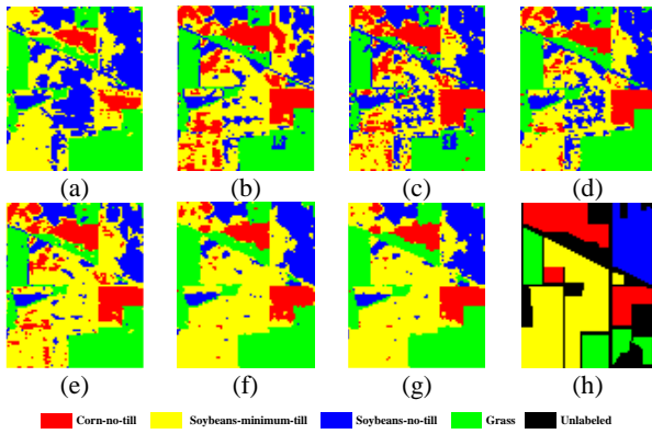
Fig. 1. The clustering results on Indian Pines image: (a) CFSFDP, (b) FCM_S1, (c) SSC, (d) S 4 C, (e) KSSC, (f) SSC-SMP, (g) KSSC-SMP, (h) ground truth.
